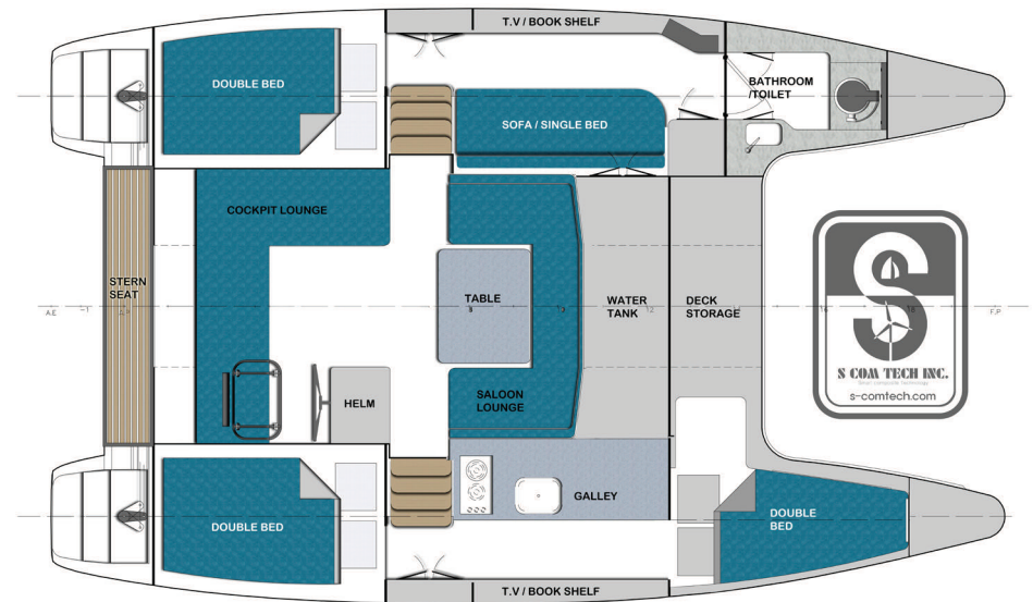
SMART CAT S280 INTERIOR PLAN - 3CABIN, 1 BATHROOM
